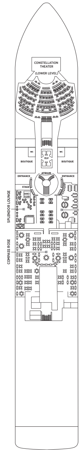
DECK 4
